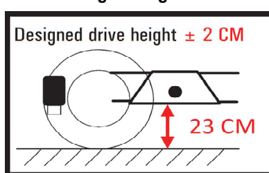
Chassis Height Range Measurement Examples
